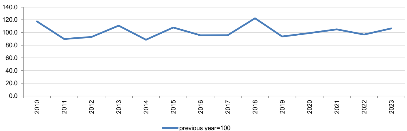
Graph 1. Annual indices of industrial production
